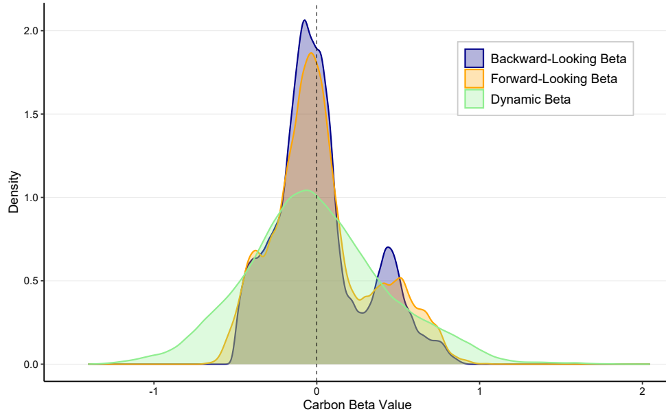
Figure 2: Carbon Beta Density
