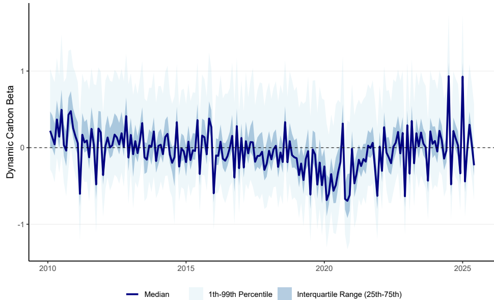
Figure 3: Carbon Beta Dynamics
